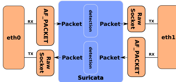
Figure 3: Suricata IPS mode in AF_PACKET
